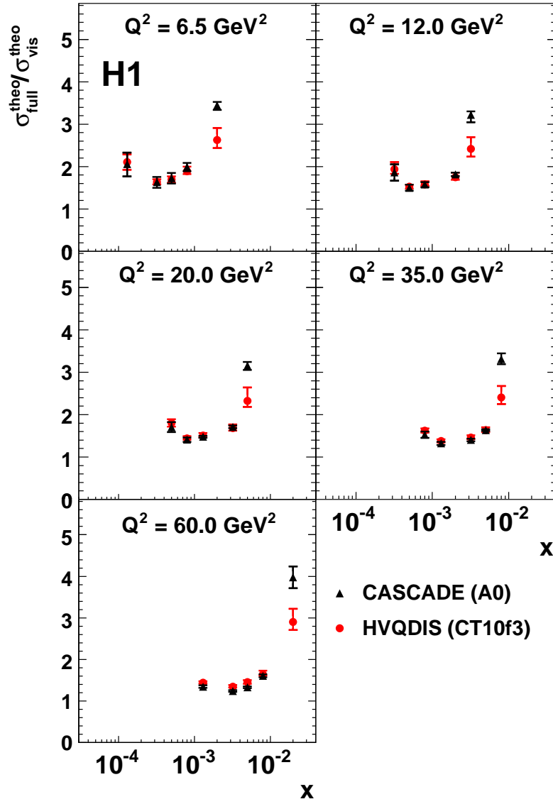
Figure 1: Extrapolation factors from the visible phase space to the total phase space for the D^* meson as determined from HVQDIS and CASCADE. The error bars show the extrapolation uncertainty which is determined by varying the theory parameters listed in tables 1 and 2 of [1].
