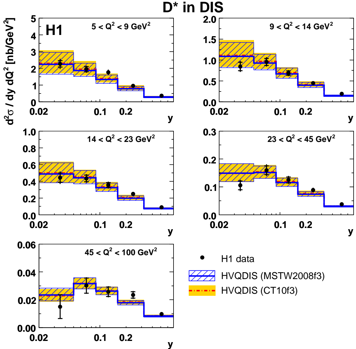
Figure 11: Double differential D^* cross section as a function of photon virtuality Q^2 and the inelasticity y . The measurements correspond to the kinematic range of 5 < Q^2 < 100 GeV 2 , 0.02 < y < 0.7 and |\eta(D^*)| < 1.8 and p_T(D^*) > 1.25 GeV. The data are shown as points, the inner error bars show the statistical error, the outer error bars represent the statistical and systematic errors added in quadrature. The data are compared to predictions by the next-to-leading order calculation HVQDIS with two different proton parton densities. The bands indicate the theoretical uncertainties (table 2).
