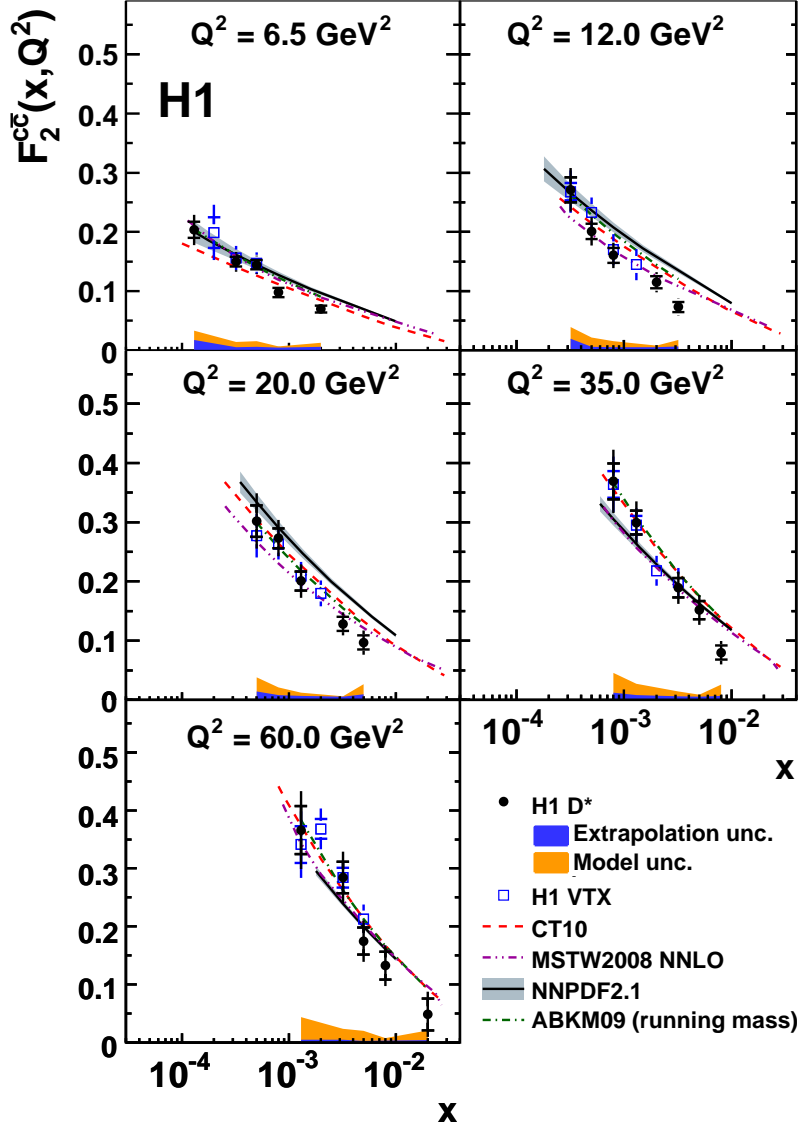
Figure 3: F_2^{c\bar{c}} as derived from D^* data with HVQDIS (points). The inner error bars show the statistical uncertainty, the outer error bar the statistical and experimental systematic uncertainty added in quadrature. The extrapolation uncertainty within the HVQDIS model is shown as blue band in the bottom of the plots. The outer (orange) band shows the model uncertainty obtained from the difference in F_2^{c\bar{c}} determined with HVQDIS and CASCADE. The data are compared to the measurement of F_2^{c\bar{c}} with the H1 vertex detector [2] (open squares) and to predictions from the global PDF fits CT10 (dashed line), MSTW08 at NNLO (dark dashed-dotted line), NNPDF2.1 (shaded band) and ABKM (light dashed-dotted line).
