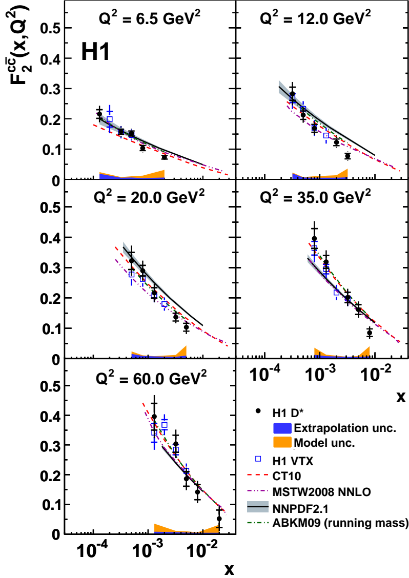
Figure 17: F_2^{c\bar{c}} as derived from D^* data with HVQDIS (points). The inner error bars show the statistical uncertainty, the outer error bar the statistical and experimental systematic uncertainty added in quadrature. The extrapolation uncertainty within the HVQDIS model is shown as blue band in the bottom of the plots. The outer (orange) band shows the model uncertainty obtained from the difference in F_2^{c\bar{c}} determined with HVQDIS and CASCADE. The data are compared to the measurement of F_2^{c\bar{c}} with the H1 vertex detector [14] (open squares) and to predictions from the global PDF fits CT10 (dashed line), MSTW08 at NNLO (dark dashed-dotted line), NNPDF2.1 (shaded band) and ABKM (light dashed-dotted line).
