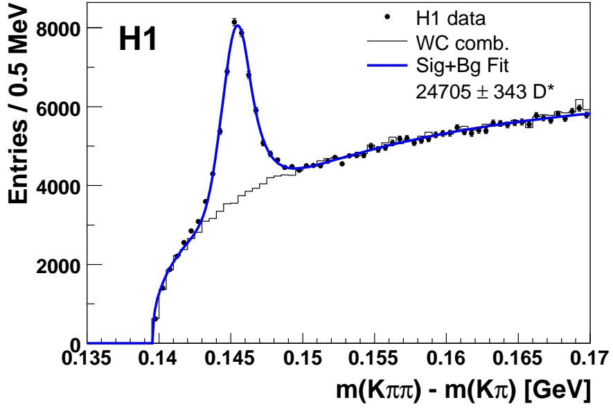
Figure 1: Distribution of the mass difference \Delta m = m(K^\mp \pi^\pm \pi_s^\pm) - m(K^\mp \pi^\pm) for D^* candidates in the kinematic range of 5 < Q^2 < 100 \text{ GeV}^2 , 0.02 < y < 0.7 , |\eta(D^*)| < 1.8 and p_T(D^*) > 1.25 \text{ GeV} . The histogram shows the wrong charge combinations, K^\pm \pi^\pm \pi_s^\mp . The solid line represents the result of the fit described in the text.
