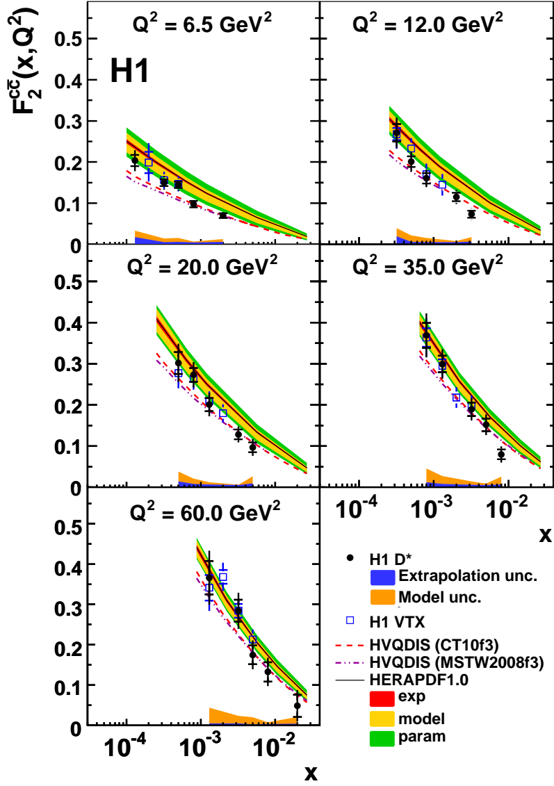
Figure 2: F_2^{c\bar{c}} as derived from D^* data with HVQDIS (points). The inner error bars show the statistical uncertainty, the outer error bar the statistical and experimental systematic uncertainty added in quadrature. The extrapolation uncertainty within the HVQDIS model is shown as blue band in the bottom of the plots. The outer (orange) band shows the model uncertainty obtained from the difference in F_2^{c\bar{c}} determined with HVQDIS and CASCADE. The data are compared to the measurement of F_2^{c\bar{c}} with the H1 vertex detector [2] (open squares), to NLO DGLAP predictions from HVQDIS with two different proton PDFs, and to the F_2^{c\bar{c}} prediction of HERAPDF1.0.
