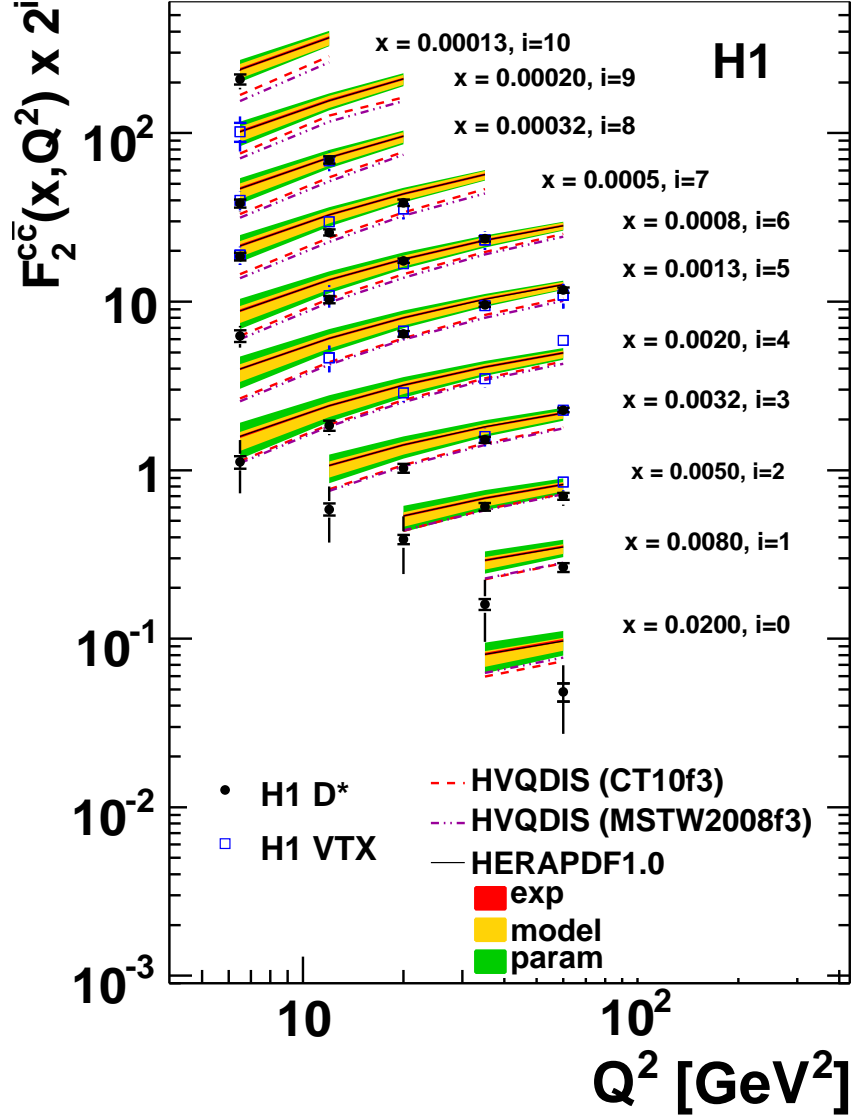
Figure 4: F_2^{c\bar{c}} as a function of Q^2 for different x , as derived from D^* data with HVQDIS (points). The inner error bars show the statistical uncertainty, the outer error bar the total uncertainty, including statistical, experimental systematic, extrapolation and model uncertainty added in quadrature. The data are compared to the measurement of F_2^{c\bar{c}} with the H1 vertex detector [2] (open squares), to NLO DGLAP predictions from HVQDIS with two different proton PDFs, and to the F_2^{c\bar{c}} prediction of HERAPDF1.0.
