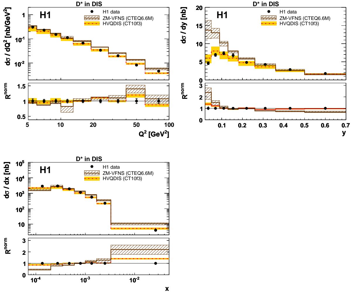
Figure 12: Differential D^* cross section as a function of photon virtuality Q^2 , the inelasticity y and Bjorken x . The measurements correspond to the kinematic range of 5 < Q^2 < 100 \text{ GeV}^2 , 0.02 < y < 0.7 , |\eta(D^*)| < 1.8 , p_T(D^*) > 1.25 \text{ GeV} with an additional cut on the D^* transverse momentum in the \gamma p centre-of-mass frame p_T^*(D^*) > 2.0 \text{ GeV} . The data are shown as points, the inner error bars show the statistical error, the outer error bars represent the statistical and systematic errors added in quadrature. The data are compared to a prediction to next-to-leading order in the ZM-VFNS and to HVQDIS. The bands indicate the theoretical uncertainties (table 2).
