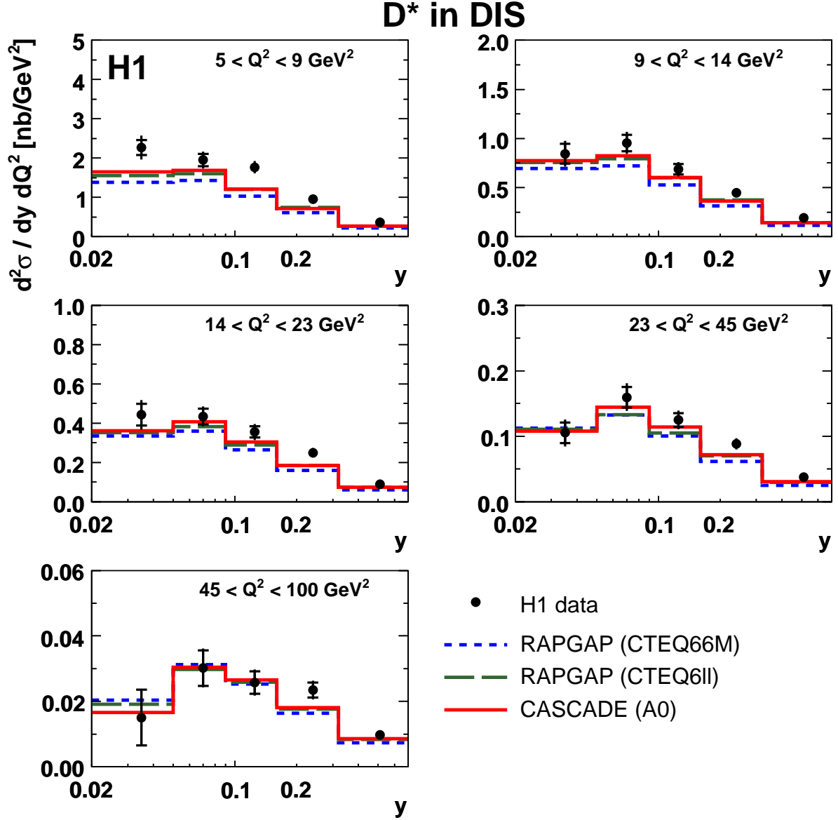
Figure 10: Double differential D^* cross section as a function of the photon virtuality Q^2 and the inelasticity y . The measurements correspond to the kinematic range of 5 < Q^2 < 100 \text{ GeV}^2 , 0.02 < y < 0.7 and |\eta(D^*)| < 1.8 and p_T(D^*) > 1.25 \text{ GeV} . The data are shown as points, the inner error bars show the statistical error, the outer error bars represent the statistical and systematic errors added in quadrature. The data are compared to predictions by the MC program RAPGAP with two different proton parton densities and by the MC program CASCADE.
