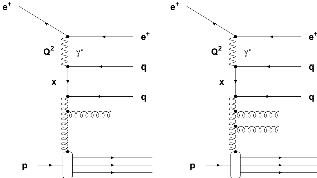
Figure 2: Examples of leading order (left) and next to leading order (right) diagrams for three-jet production in DIS at HERA with one and two radiated gluons, respectively.
