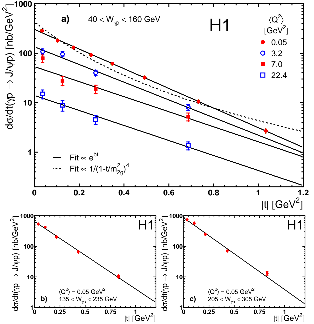
Figure 7: Differential cross section d\sigma/dt for elastic J/\psi production as a function of |t| a) in four bins of Q^2 in the range 40 < W_{\gamma p} < 160 \text{ GeV} . \langle Q^2 \rangle indicates the bin centre value in the Q^2 range considered. The inner error bars show the statistical error, while the outer error bars show the statistical and systematic uncertainties added in quadrature. The solid lines show fits to the data of the form d\sigma/dt \propto e^{bt} . The dashed curve shows the result of a fit proposed by Frankfurt and Strikman [8]. Figures b) and c) show the photoproduction measurements in the ranges 135 < W_{\gamma p} < 235 \text{ GeV} and 205 < W_{\gamma p} < 305 \text{ GeV} .
