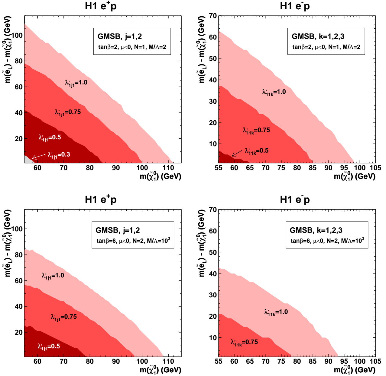
Figure 5: Excluded regions at the 95 % CL in the \Delta m = m(\tilde{e}_L) - m(\tilde{\chi}_1^0) and m(\tilde{\chi}_1^0) plane for various values of \lambda'_{1j1} ( j = 1, 2 ) and \lambda'_{11k} ( k = 1, 2, 3 ).
