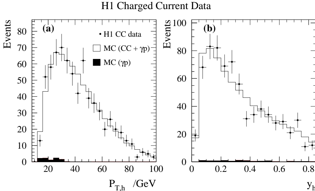
Figure 2: Distributions of (a) P_{T,h} and (b) y_h for CC data (solid points) and simulation (solid line). The filled histograms show the photoproduction contribution.
