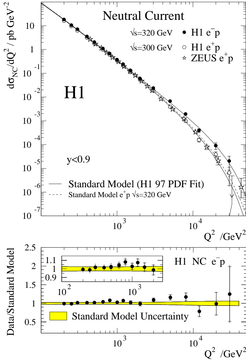
Figure 5: The Q^2 dependence of the NC cross section d\sigma_{\text{NC}}/dQ^2 is shown for the H1 e^-p data (solid points) and e^+p measurements (open points) from H1 [2] and ZEUS [3]. The data are compared with the Standard Model expectation determined from the H1 97 PDF Fit including the H1 e^+p data. The dashed curve shows the influence of an increased centre-of-mass energy on the e^+p cross section. The ratio of the e^-p data to the Standard Model expectation is shown in the lower figure. The Standard Model uncertainty is shown as the shaded band. The inner error bars represent the statistical error, and the outer error bars show the total error. The normalisation uncertainties are not included in the error bars.
