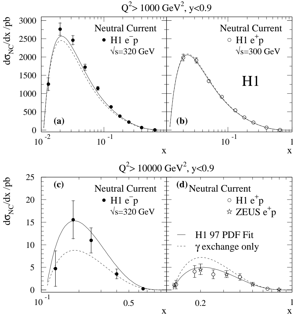
Figure 3: The NC cross sections d\sigma_{\text{NC}}/dx for the e^-p data are shown in (a) for Q^2 > 1000 \text{ GeV}^2 and in (c) for Q^2 > 10000 \text{ GeV}^2 . The H1 e^+p cross sections [2] are shown in (b) and (d) for Q^2 > 1000 \text{ GeV}^2 and 10000 \text{ GeV}^2 respectively. In addition the ZEUS e^+p data [3] are shown for Q^2 > 10000 \text{ GeV}^2 . The solid curves show the Standard Model expectation based on the H1 97 PDF Fit. The dashed curves show the contribution of photon exchange only. All cross sections are shown for y < 0.9 . The inner error bars represent the statistical error, and the outer error bars show the total error. The normalisation uncertainties are not included in the error bars.
