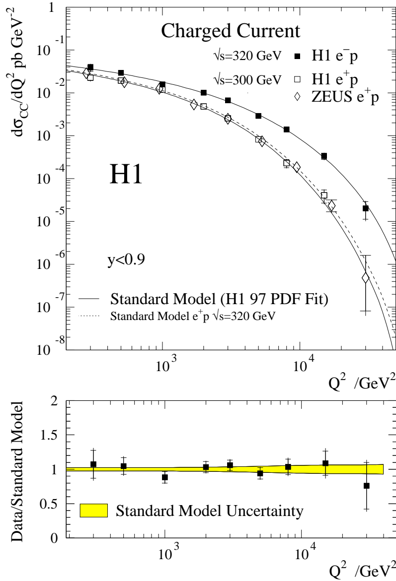
Figure 6: The Q^2 dependence of the CC cross section d\sigma_{CC}/dQ^2 is shown for the e^-p data (solid points) and e^+p measurements (open points) from H1 and ZEUS [3]. The data are compared with the Standard Model expectation determined from the H1 97 PDF Fit including the H1 e^+p data. The dashed curve shows the influence of an increased centre-of-mass energy on the e^+p data. The ratio of the e^-p data to the Standard Model expectation is shown in the lower figure. The Standard Model uncertainty is shown as the shaded band. The inner error bars represent the statistical error, and the outer error bars show the total error. The normalisation uncertainties are not included in the error bars.
