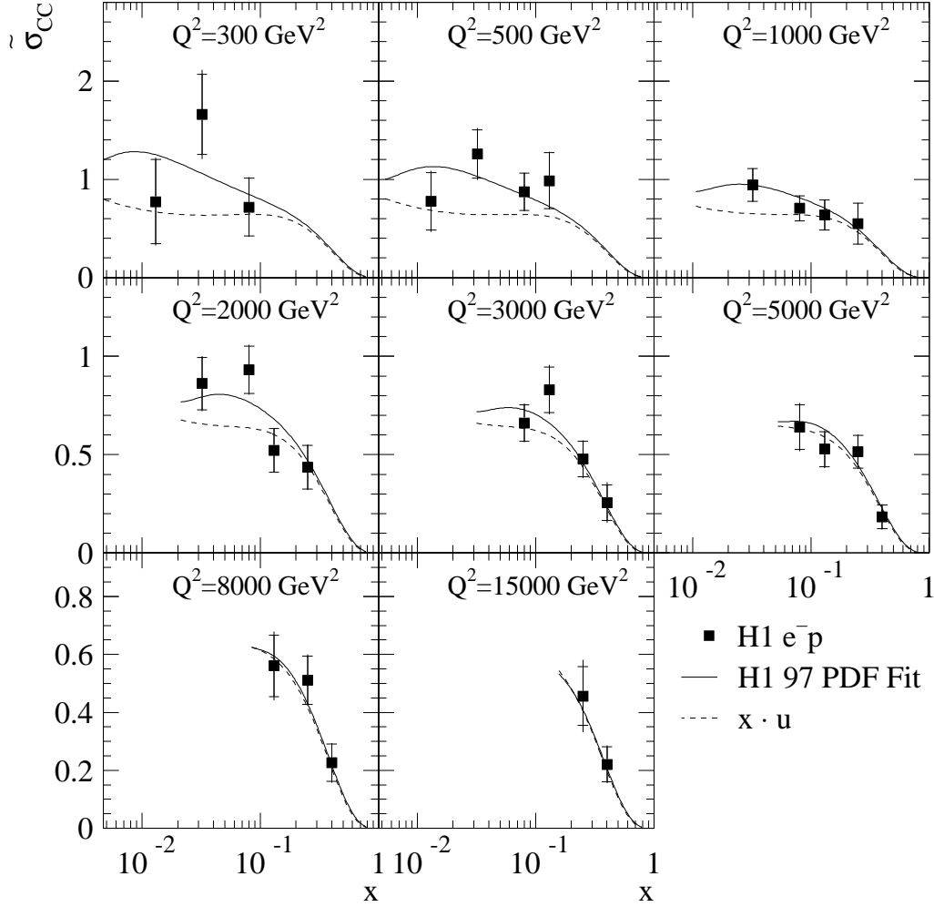
Figure 9: The CC reduced cross section \tilde{\sigma}_{CC}(x, Q^2) is shown for e^-p scattering at \sqrt{s} \approx 320 GeV (solid points). The data are compared with the H1 97 PDF Fit. The inner error bars represent the statistical error, and the outer error bars show the total error. The normalisation uncertainty is not included in the error bars.
