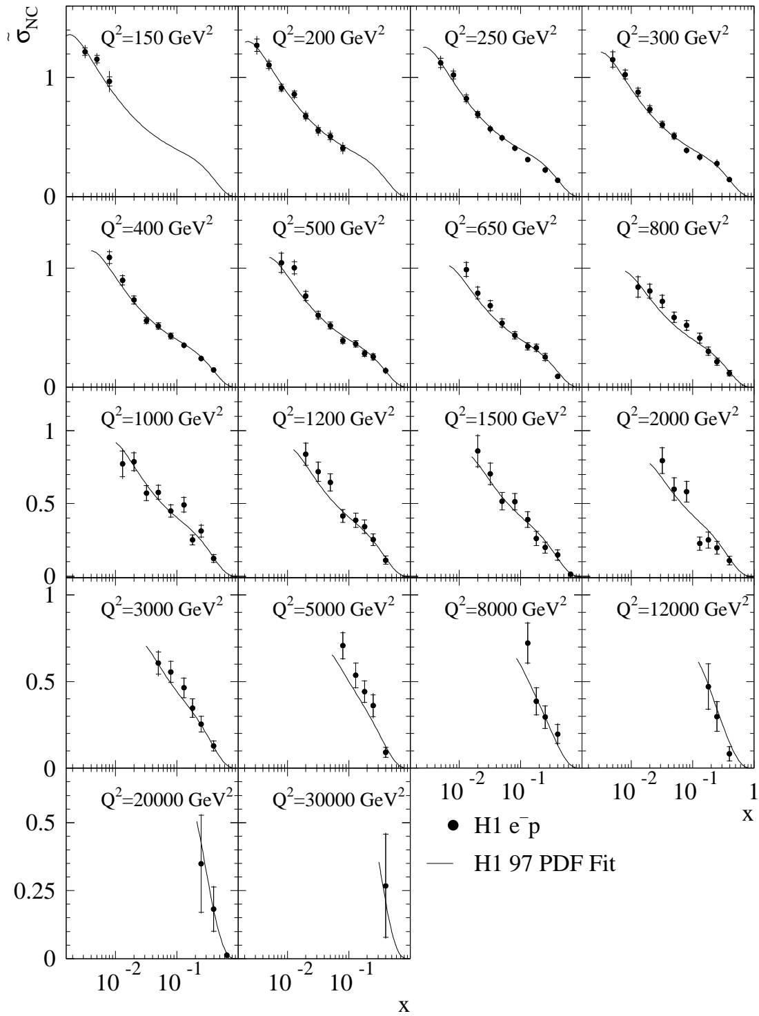
Figure 7: The NC e^-p reduced cross section \tilde{\sigma}_{NC}(x, Q^2) is compared with the H1 97 PDF Fit. The inner error bars represent the statistical error, and the outer error bars show the total error. The normalisation uncertainty is not included in the error bars.
