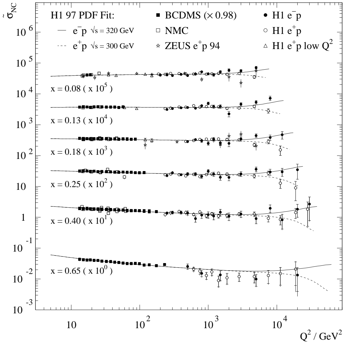
Figure 8: The NC reduced cross section \tilde{\sigma}_{NC}(x, Q^2) is shown at high x compared with the H1 97 PDF Fit. The e^-p data with \sqrt{s} \approx 320 GeV (solid circles) are compared with the H1 e^+p data at \sqrt{s} \approx 300 GeV (open circles), ZEUS e^+p data [3], and fixed target data from BCDMS [17] and NMC [16]. The solid curves represent the Standard Model expectation based on the H1 97 PDF Fit. The inner error bars represent the statistical error, and the outer error bars show the total error. The normalisation uncertainties are not included in the error bars.
