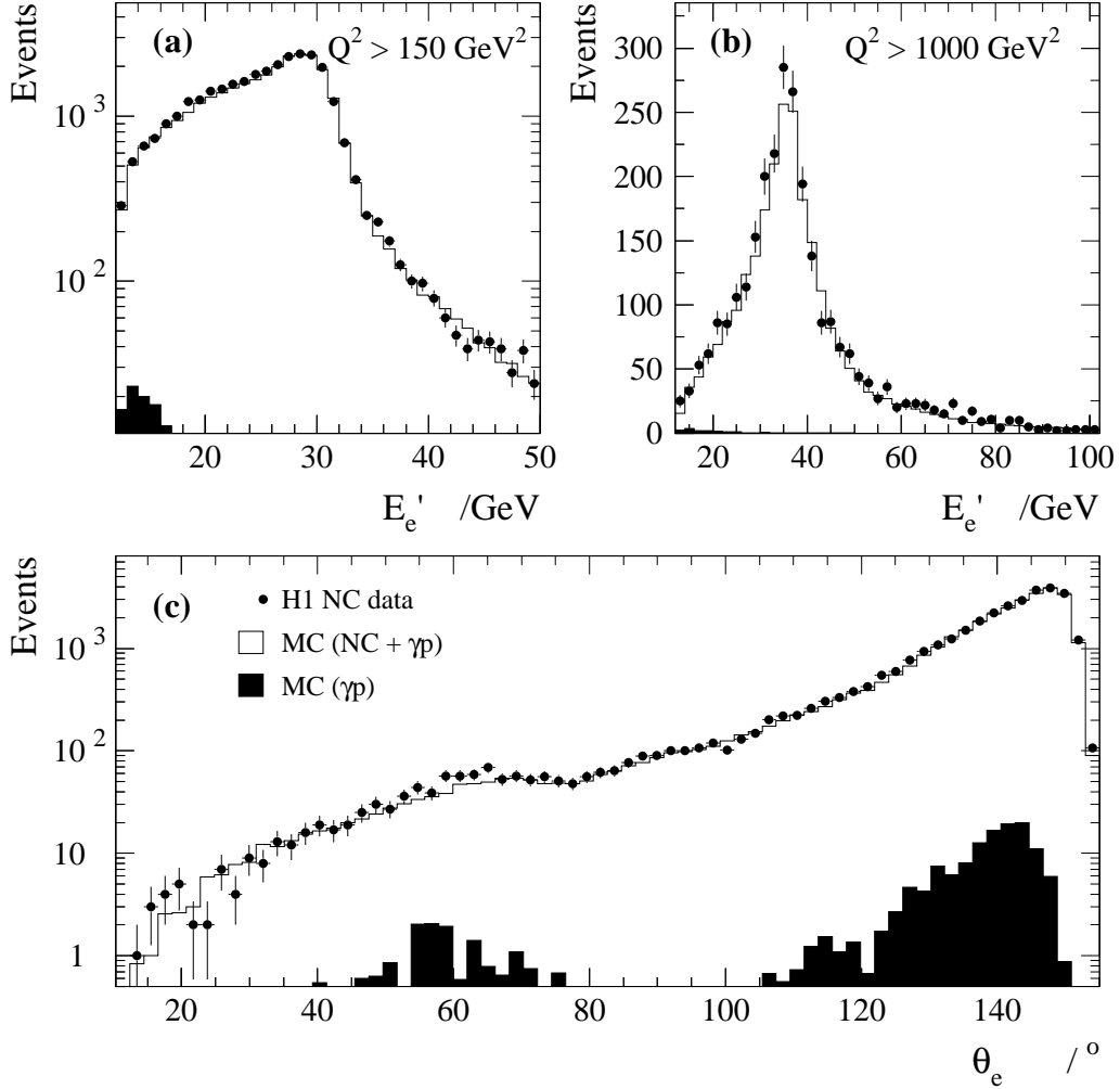
Figure 1: Distributions of (a) E'_e for Q^2 > 150 \text{ GeV}^2 , (b) E'_e for Q^2 > 1000 \text{ GeV}^2 and (c) \theta_e for NC data (solid points) and simulation (solid line). The filled histograms show the photoproduction contribution.
