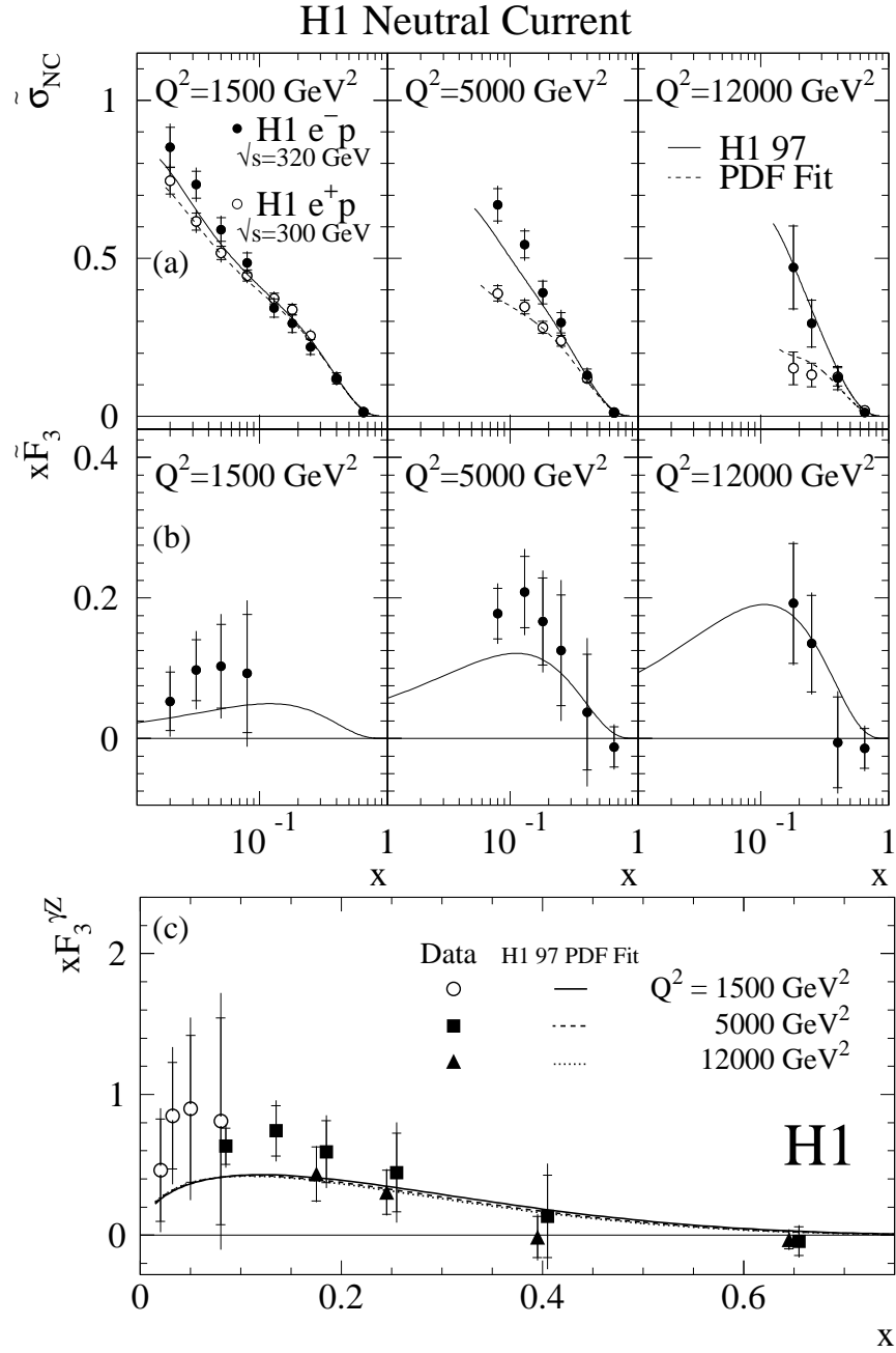
Figure 10: The NC reduced cross section \tilde{\sigma}_{NC}(x, Q^2) is compared with the H1 97 PDF Fit for three different Q^2 values (a). The e^-p data with \sqrt{s} \approx 320 \text{ GeV} (solid points) are compared with the H1 e^+p data at \sqrt{s} \approx 300 \text{ GeV} (open points). The structure function x\tilde{F}_3 is compared with the H1 97 PDF Fit (b). The structure function x\tilde{F}_3^{\gamma Z} is compared with the H1 97 PDF Fit (c). In all figures the inner error bars represent the statistical error, and the outer error bars show the total error. The normalisation uncertainties of the e^-p and e^+p data sets are included in the systematic errors.
