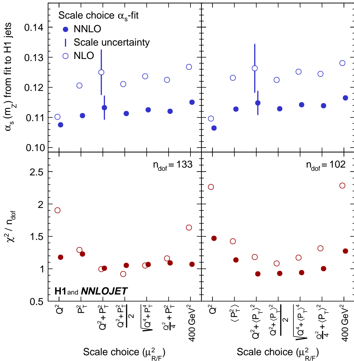
H1 inclusive jets
