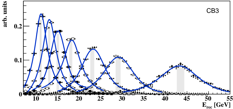
Figure 8.21: Distributions of reconstructed jet energies for simulated jets incident on the CB3 . The generated energies are shown as dashed grey areas. Fits to equation (8.1) are shown with blue lines.
