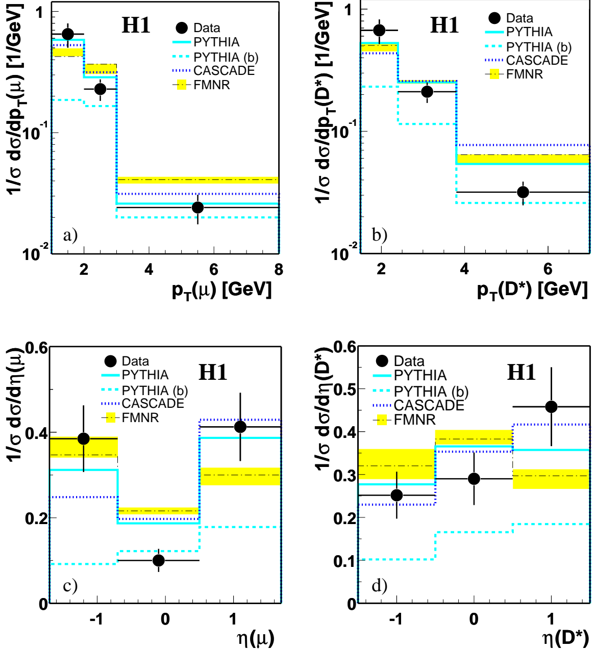
Figure 4: Normalised differential D^*\mu cross sections as functions of the transverse momenta and the pseudorapidities of muons (a,c) and D^* mesons (b,d). The data (points) are compared with the prediction of the NLO calculation FMNR and the LO-ME+PS QCD models PYTHIA and CASCADE. A beauty fraction of 45% as obtained from the measured cross sections is used in the calculations. The error bands for FMNR are obtained as described in table 4. The PYTHIA b quark contribution is indicated separately. The experimental systematic uncertainties for the normalised distributions are negligible compared to the statistical errors.
