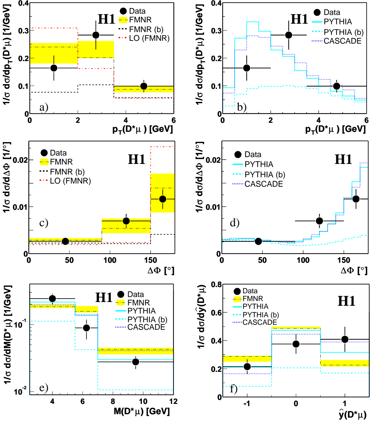
Figure 5: Normalised differential D^*\mu cross sections for a,b) the transverse momenta p_T(D^*\mu) , c,d) the azimuthal angle difference \Delta\Phi , e) the invariant mass M(D^*\mu) and f) the rapidity \hat{y}(D^*\mu) of the D^*\mu -pairs. The data are compared to the prediction of the LO and NLO calculations FMNR (a,c,e,f) and to the Monte Carlo models PYTHIA and CASCADE (b,d,e,f). The error bands for FMNR are obtained as described in table 4. A beauty fraction of 45% as obtained from the measured cross sections is used in the calculations. The FMNR (a,c) and PYTHIA (b,d,e,f) b quark contributions are indicated separately. The experimental systematic uncertainties for the normalised distributions are negligible compared to the statistical errors.
