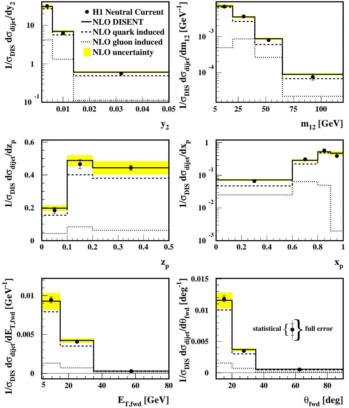
Figure 8: Distributions of y_2 , m_{12} , z_p , x_p , E_{T,fwd} and \theta_{fwd} in NC events with p_T^{lept} > 25 GeV and 0.03 < y < 0.85 determined with the modified Durham algorithm. The events satisfy the cuts y_2 > 0.002 and 10^\circ < \theta_{jet} < 140^\circ . Also shown are perturbative QCD calculations in NLO obtained with DISENT combined with a correction for hadronization effects. The shaded area shows the hadronization uncertainties and the renormalization scale uncertainties of the NLO calculations added in quadrature. In addition, the jet distributions obtained for quark- and gluon-induced processes are shown separately.
